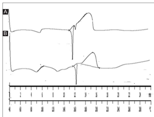
Fig. 2: Differential scanning calorimetric thermogram. DSC thermogram of drug (A) and formulation (B).
